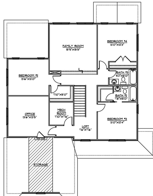
FLOOR PLAN SECOND FLOOR
