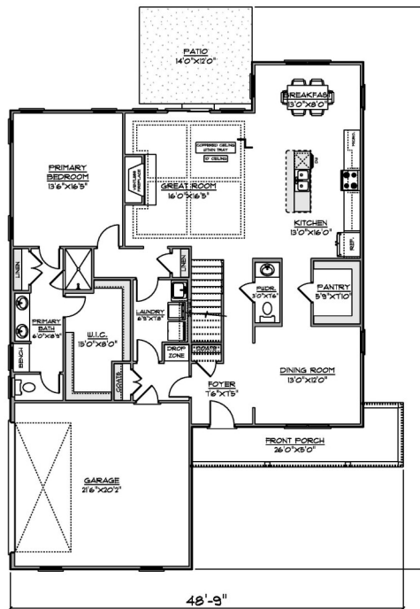
FLOOR PLAN FIRST FLOOR
