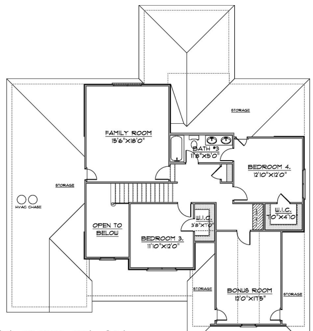
FLOOR PLAN SECOND FLOOR
