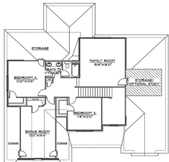
FLOOR PLAN SECOND FLOOR
