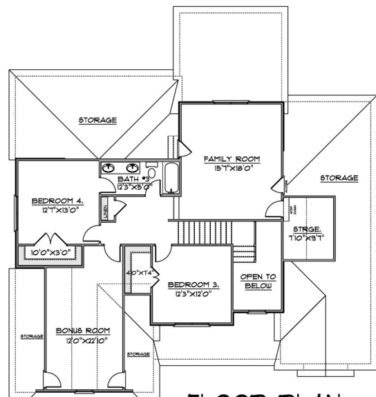
FLOOR PLAN SECOND FLOOR
