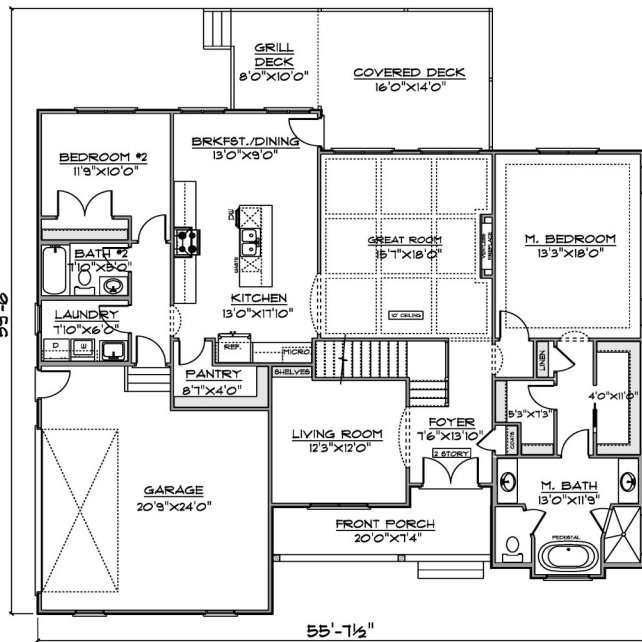
FLOOR PLAN FIRST FLOOR
