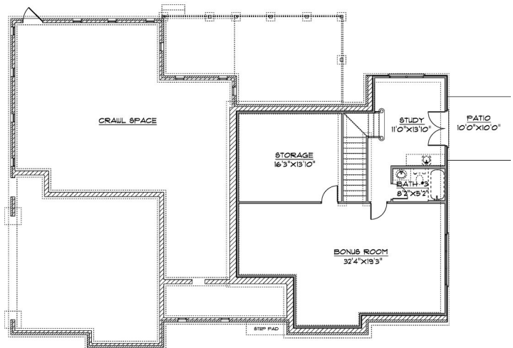
BASEMENT PLAN
