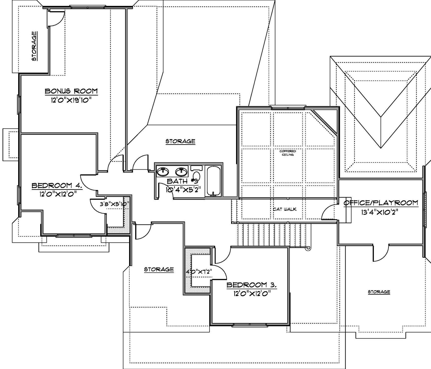
FLOOR PLAN SECOND FLOOR
