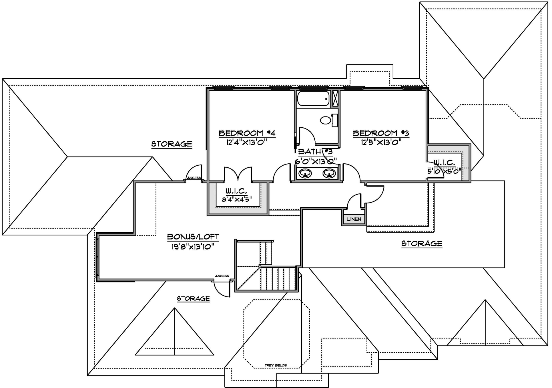
FLOOR PLAN SECOND FLOOR
