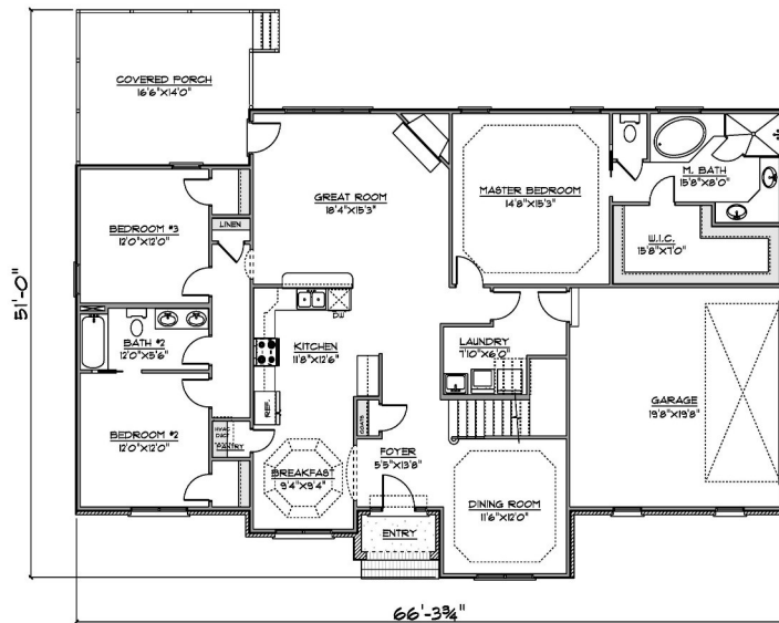
FLOOR PLAN FIRST FLOOR
